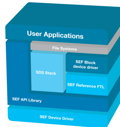
Figure 2: Software-Enabled Flash technology API
